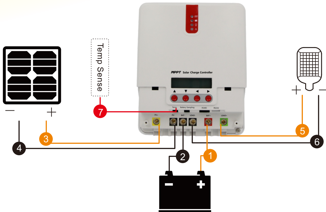
Figure 2-3 Wiring
